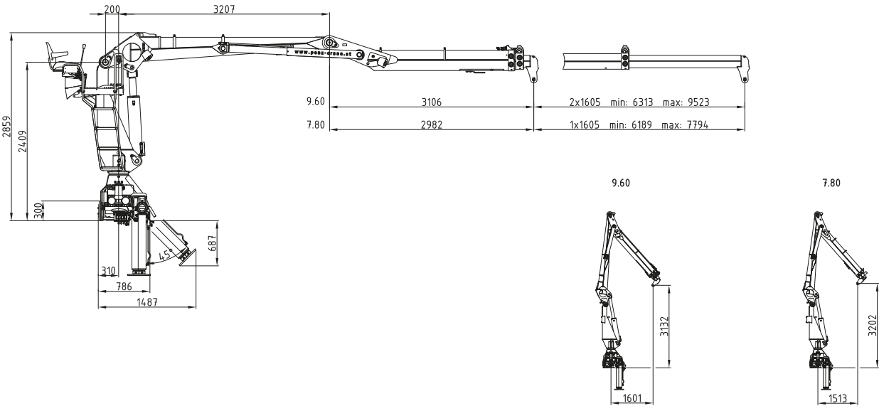
Sockel Crane base
