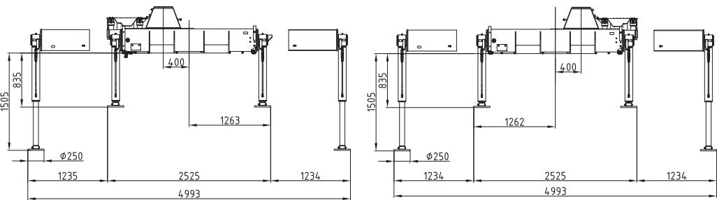
Sockel Crane base
