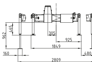
Sockel Crane base
