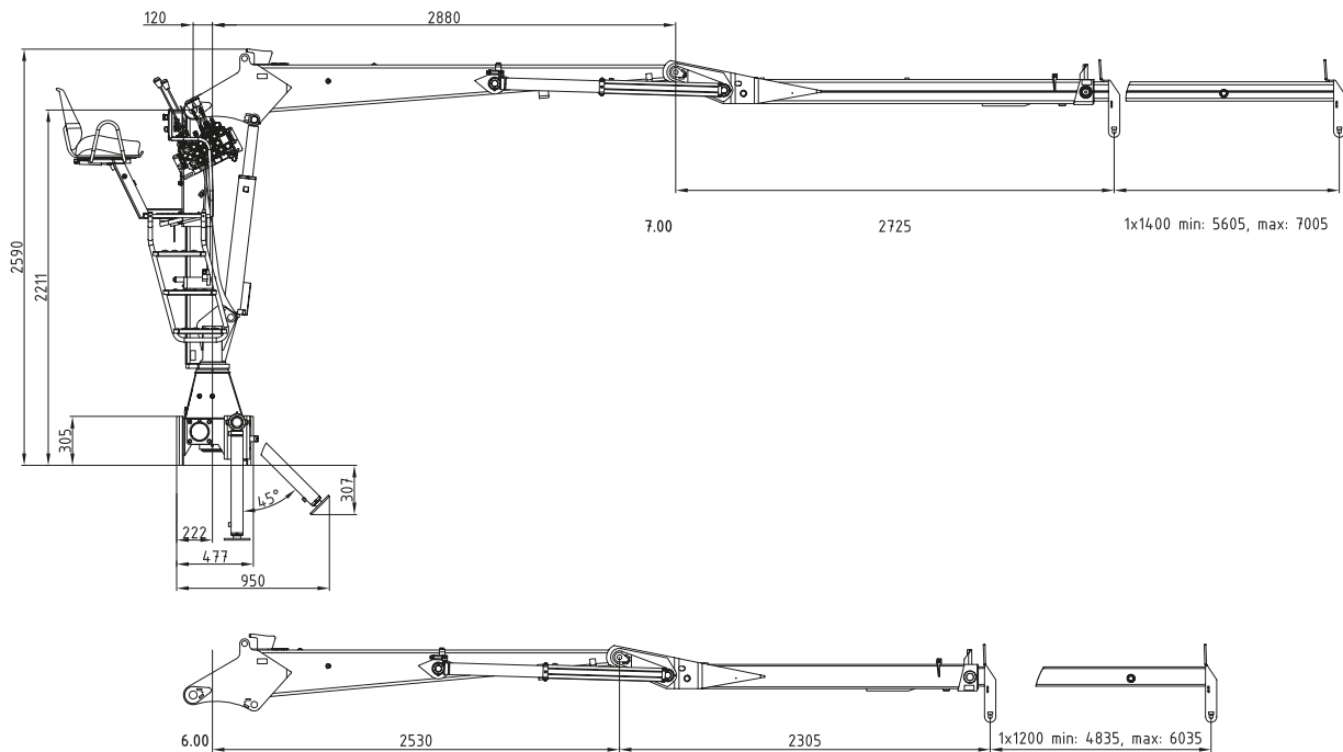
Sockel Crane base
