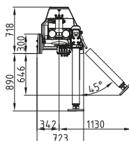
Kransockel 3800mm Crane base 3800mm
