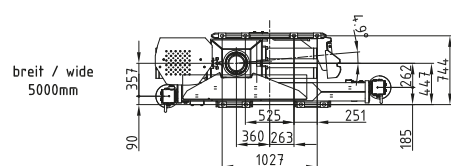
Kransockel *Kransockel 5000mm Crane base *Crane base 5000mm
