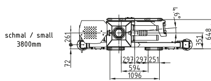
Kransockel 3800mm Crane base 3800mm
