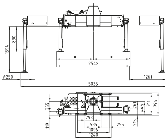
Kransockel breit Crane base wide
