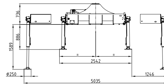
Kransockel breit Crane base wide
