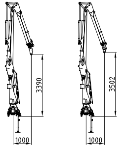
Kransockel schmal Crane base small
