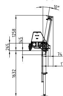
Sockel schmal Crane base small
