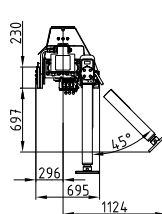
Kransockel schmal Crane base small
