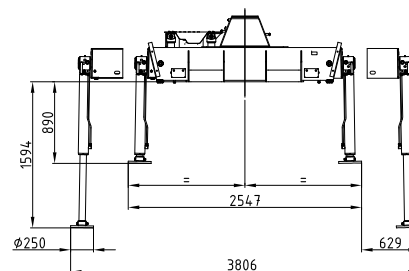
Sockel schmal Crane base small
