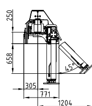
Kransockel breit Crane base wide
