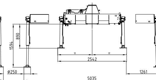
Sockel breit Crane base wide
