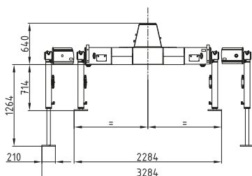
Kransockel mittig Crane base centered
