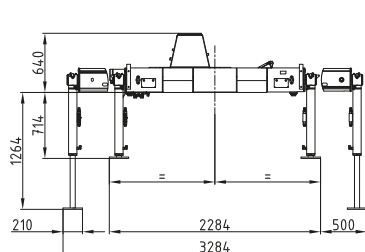
Kransockel Standard Crane base standard
