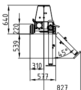
Kransockel Standard Crane base standard
